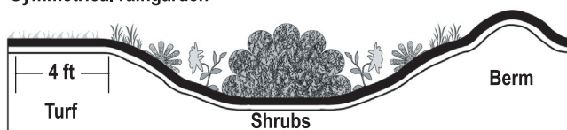
Figure 1. Typical asymmetrical and symmetrical raingardens (adapted from Barr Engineering Company, 2001).
