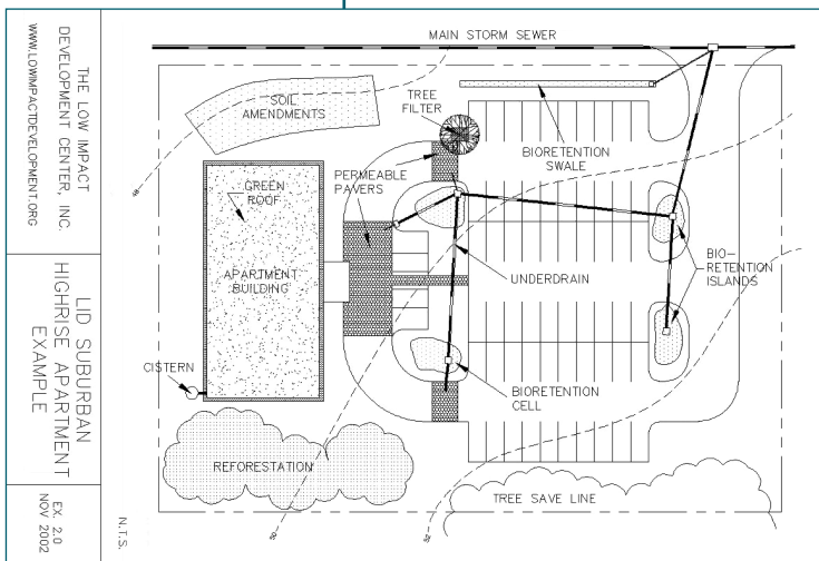
Figure 3. Parking lot design showing several rain garden cells connected with underground drains. (Source: Low Impact Development Center Inc.)
