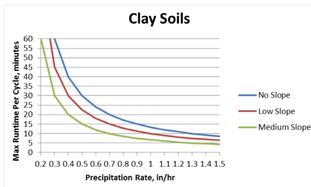
Figure 1. Maximum runtime per cycle graph for clay soils.
