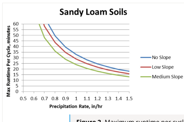
Figure 2. Maximum runtime per cycle graph for sandy loam soils.
